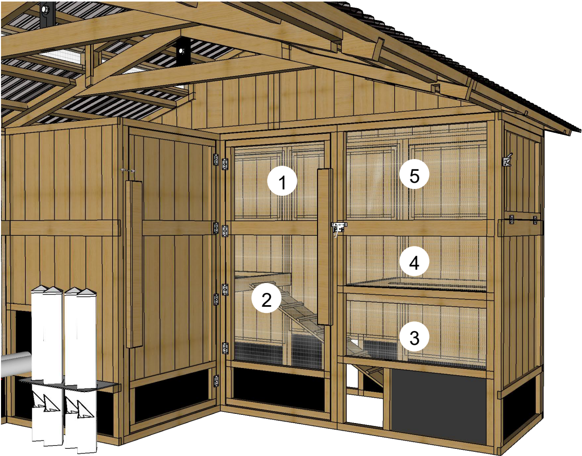
All 5 panels on the mid wall are unique. * Note that panels allow for about 3/16 gap all around for manufacturing tolerances and ventilation.
