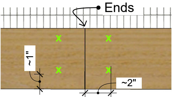
2x4 Screw Pattern
