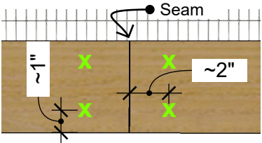
2x4 Screw Pattern
